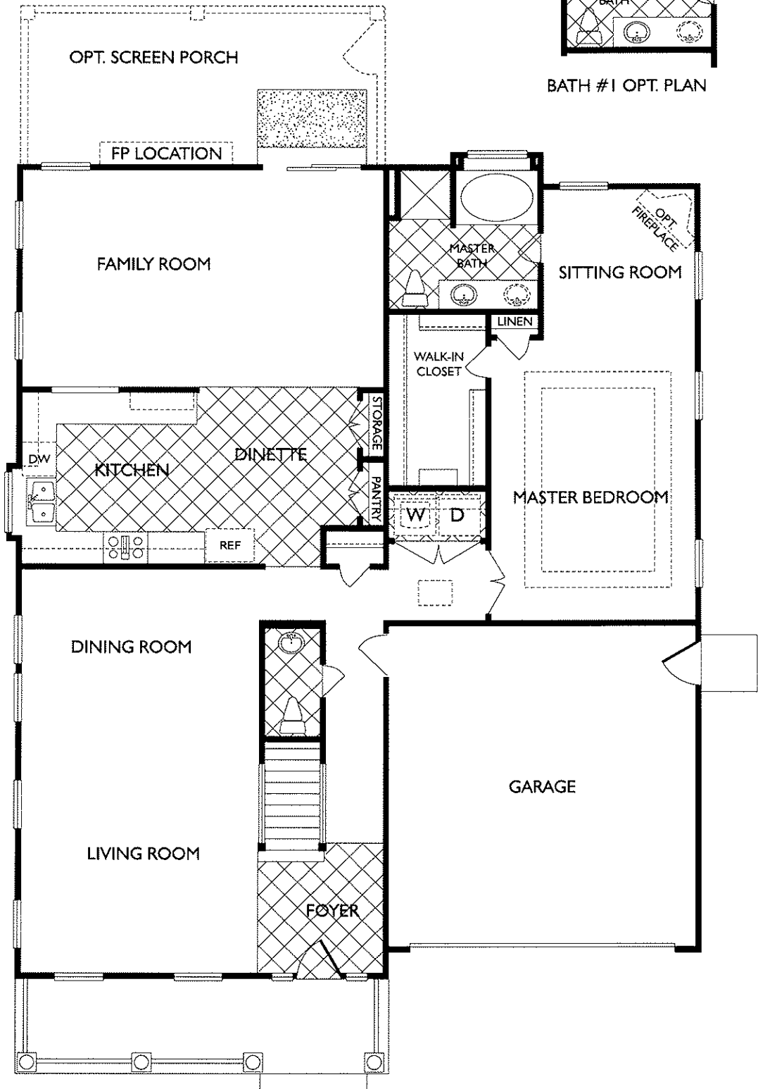
FIRST FLOOR PLAN MODEL-KFF-E-1070 MODEL-KFF-E-1071
